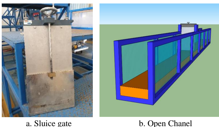
Figure 3 Physical Model of Open Channel
